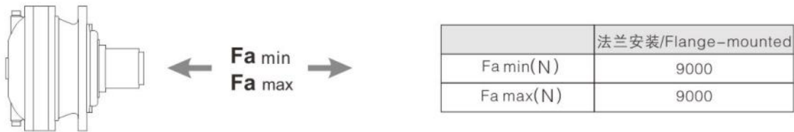
Axial force (Output shafts)
