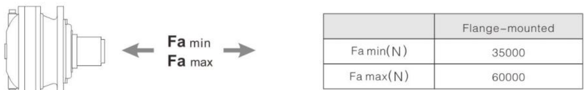
Axial force (Output shafts)
